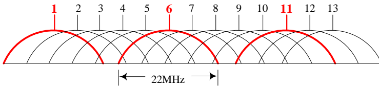
Figure 1: Channel planning of 2.4GHz spectrum
