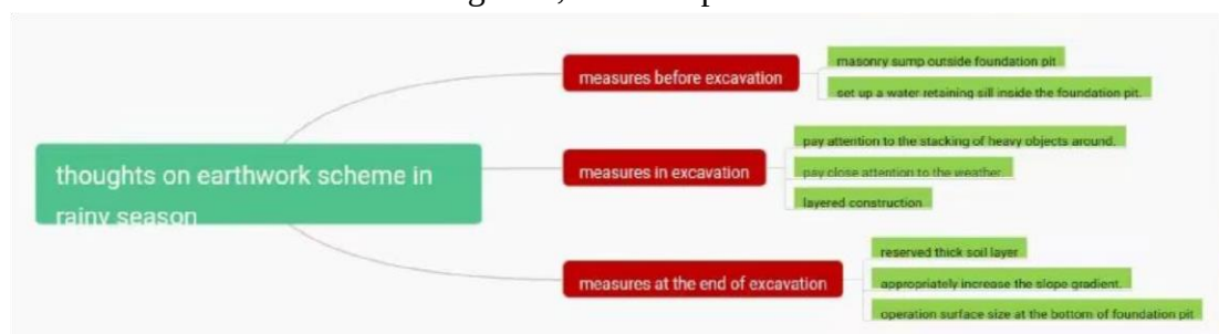
Figure 5 Idea diagram of earthwork measures
