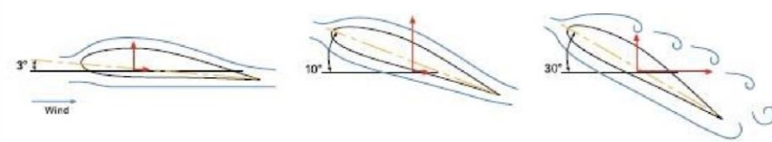
Figure 4 Blade at low, medium & high angles of attack(WE HANDBOOK) [3]
