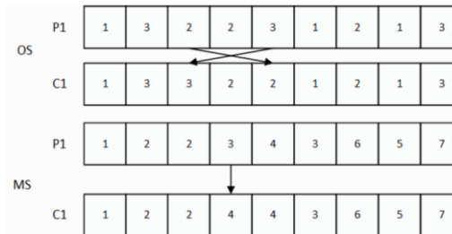
Figure 8: Mutation operation.
