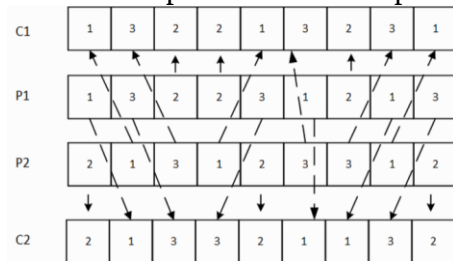
Figure 7: POX cross algorithm.
