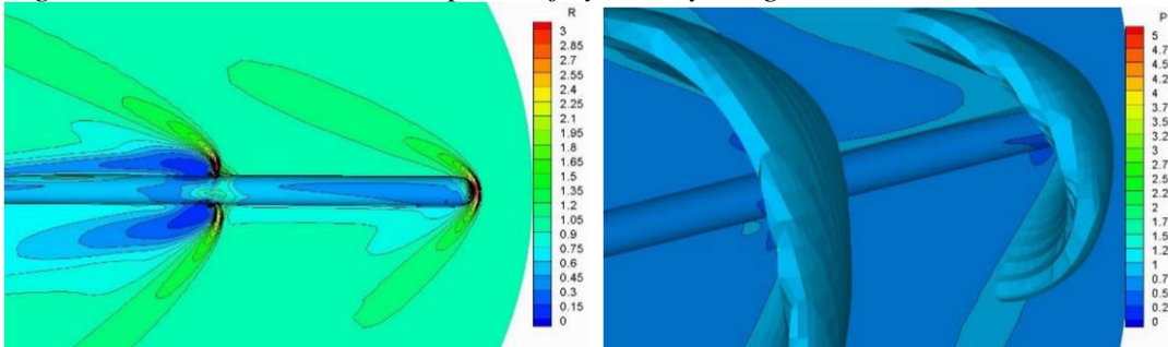
Figure 4: Density distribution on symmetry plane Figure 5: Isometric pressure changes
