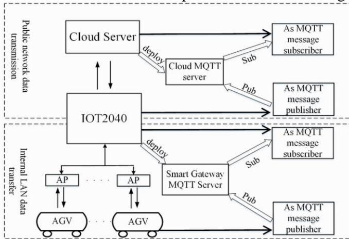
Figure 4: Structure block diagram of gateway data transfer module.
