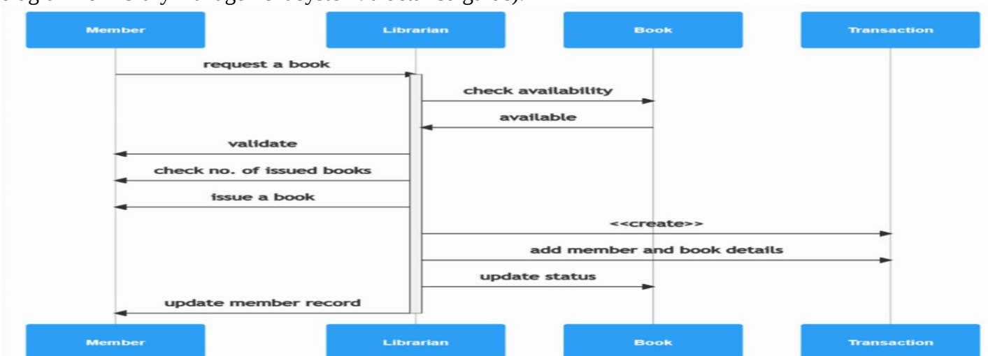
Figure 3: PC component family library management system management sequence diagram
