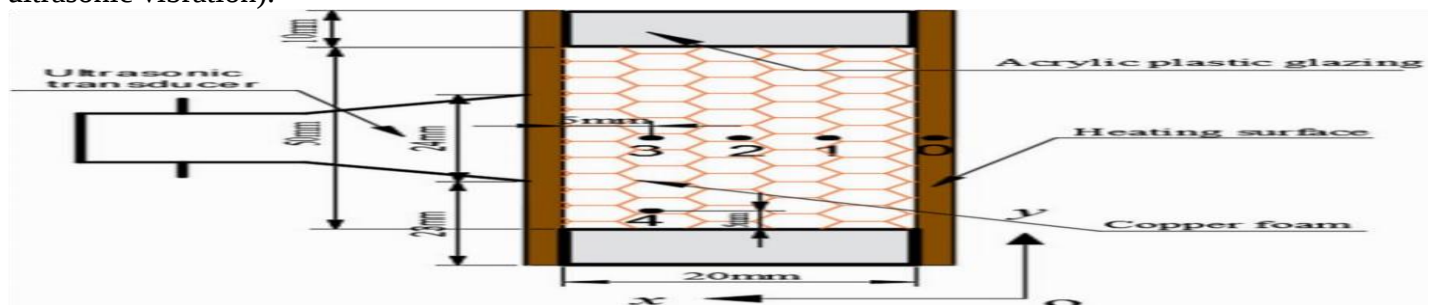
Figure 5: Schematic diagram of measuring point layout
