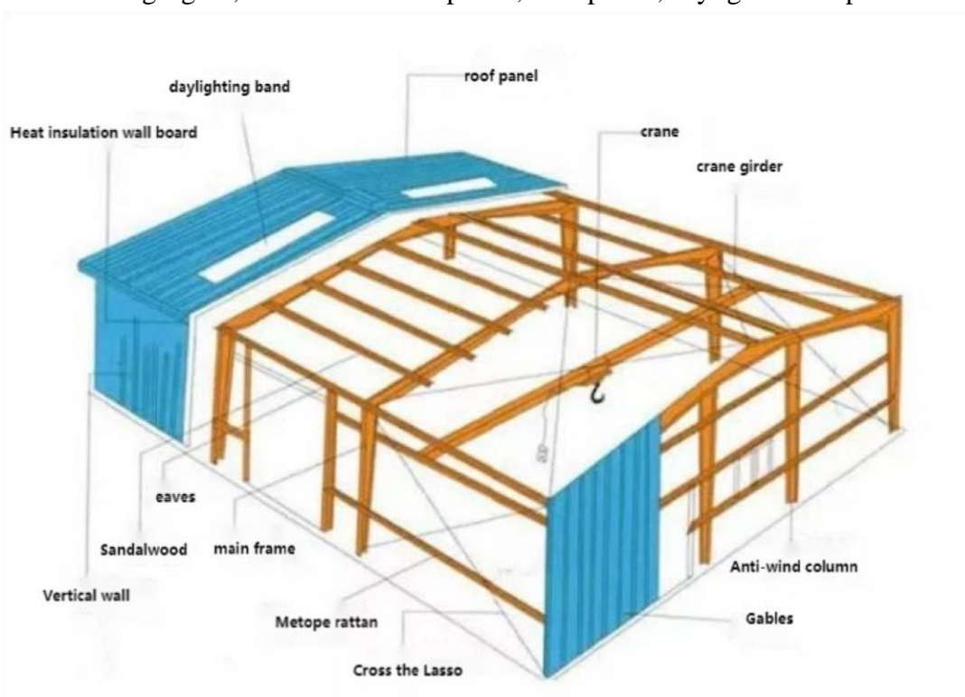
Figure 1: Construction technology of light steel structure roof purlin of portal steel frame
