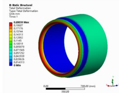
Figure 8: Thermal deformation of the guide sleeve
