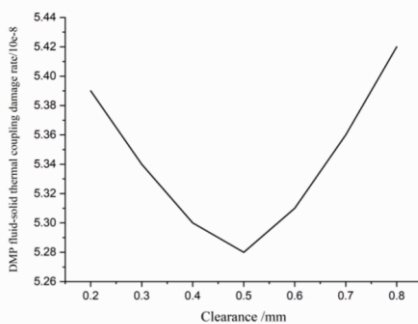
Figure 11: Clearance optimization diagram
