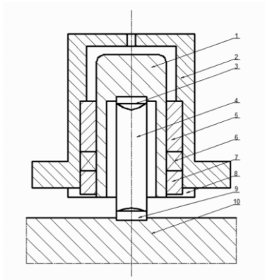
(1) Plunger, (2) cylinders, (3) hinge on the ball, (4) connecting rod, (5) guide sleeve, (6) seal, (7) pressing sleeve, (8) plunger gland, (9) under the spherical hinge, (10) walking beam.
