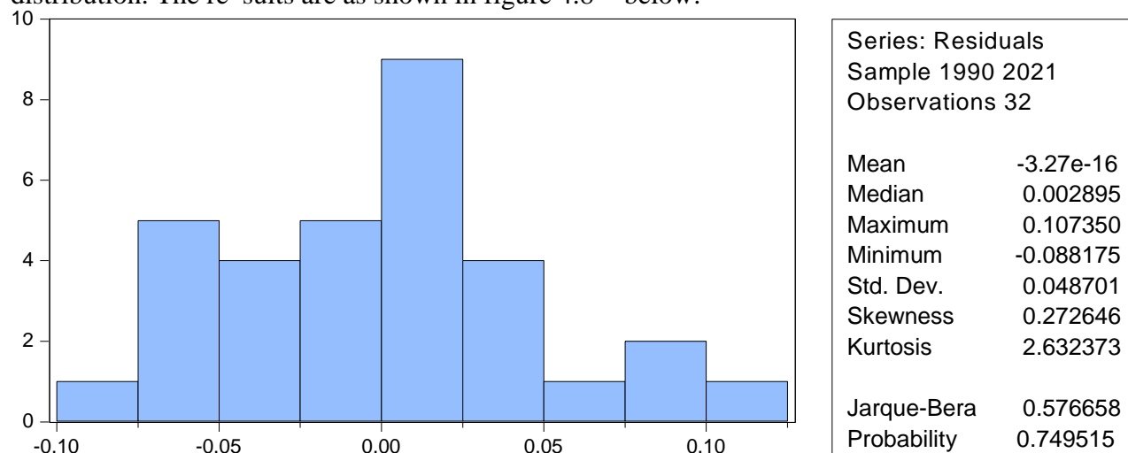
Figure 4.8 : Normality test
