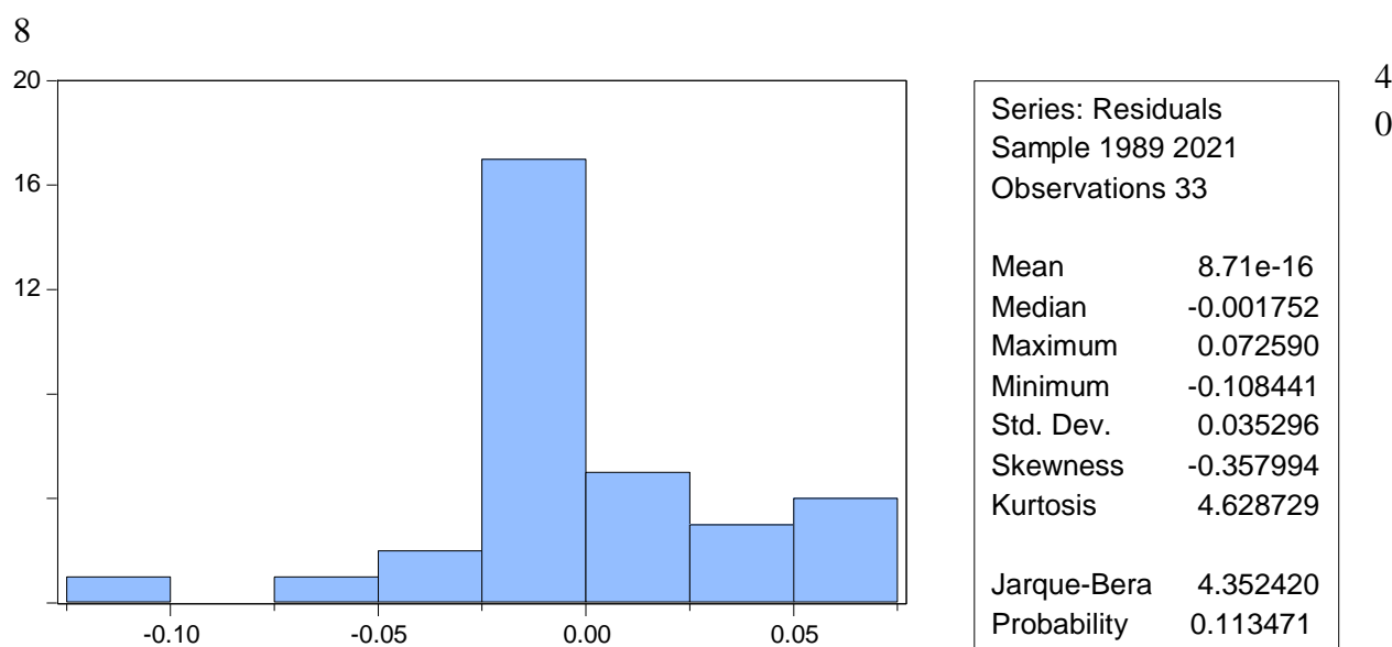
Figure: 4.16: Normality Test for MASR
