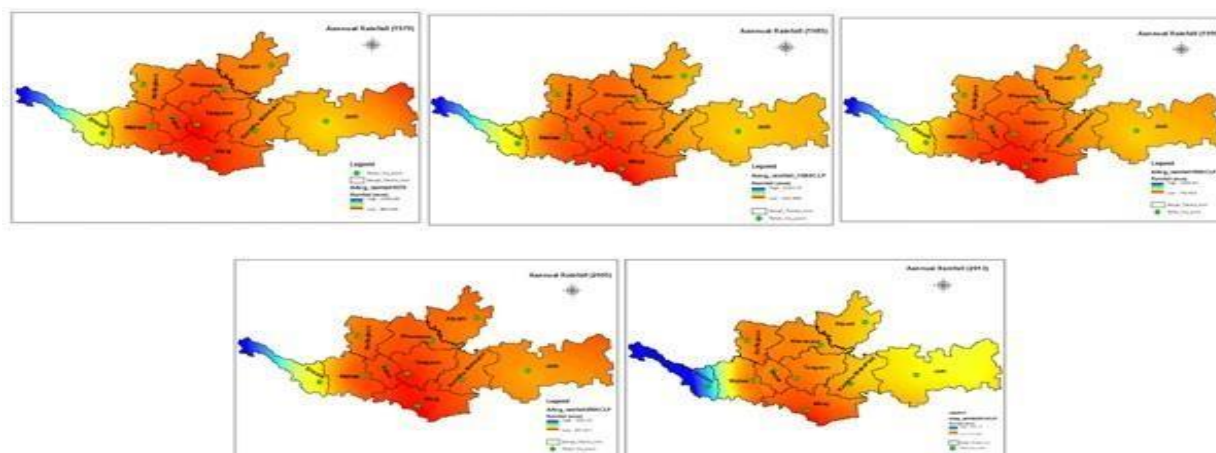
Fig.3 Annual Rainfall (1979,1985,1995,2005,2013)
