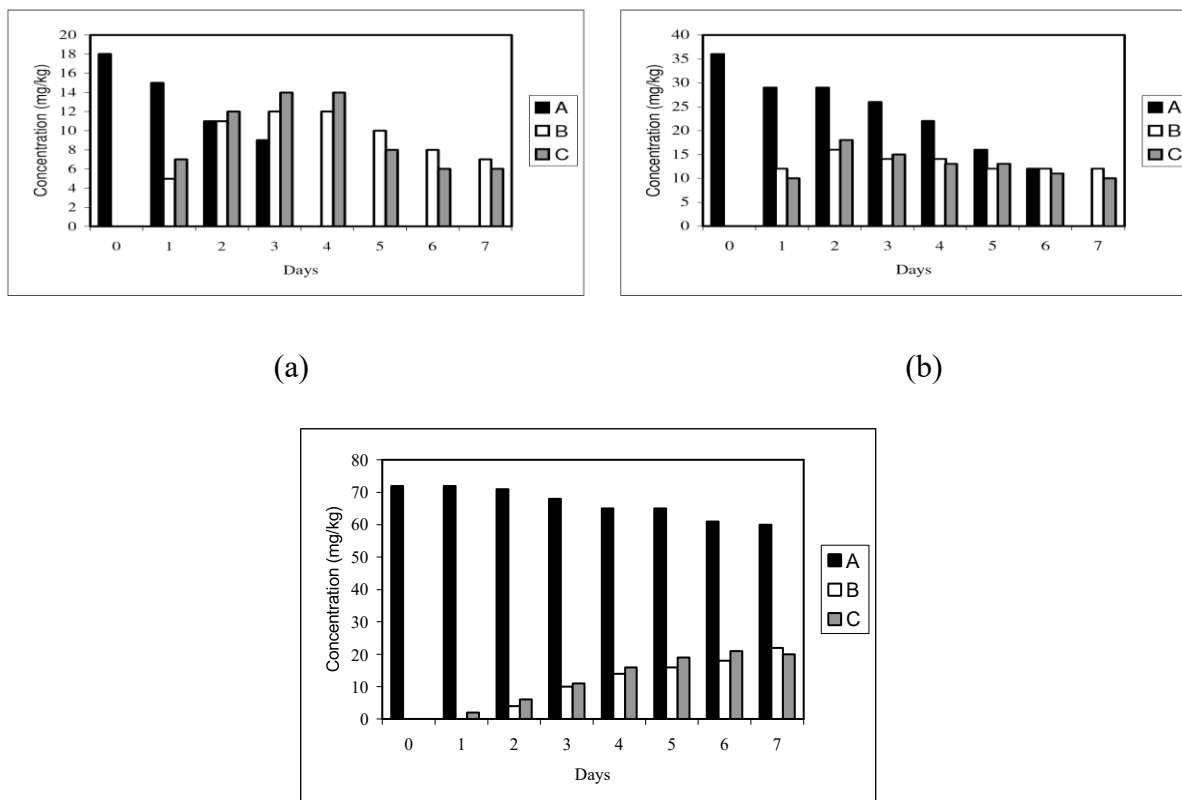
(c) Figure 4. Concentration of intermediates found during the bioremediation of Fenvlalerate amended soil (a) 25 mg/l Fenvlalerate amended soil (b) 50 mg/l Fenvlalerate amended soil (c) 100 mg/l Fenvlalerate amended soil where A = fenvlalerate, B = 4-chloro-alpha (1-methylethyl) benzene acetic acid and C = alpha-cyano-3-phenoxybenzyl alcohol.
