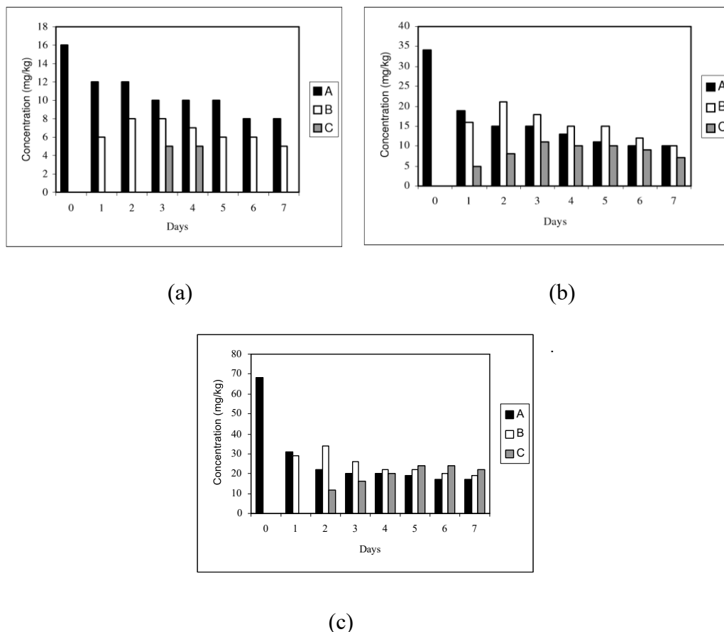
Figure 5. Concentration of intermediates found during the bioremediation of TBEE amended soil (a) 25 mg/l TBEE amended soil (b) 50 mg/l TBEE amended soil (c) 100 mg/l TBEE amended soil where A = TBEE, B = Trichlopyr acid and C = TCP.
