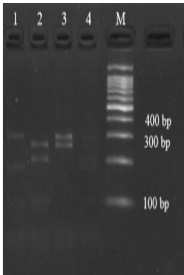
Fig. 2. Restriction profiles obtained after digestion of the HhaI enzyme.
