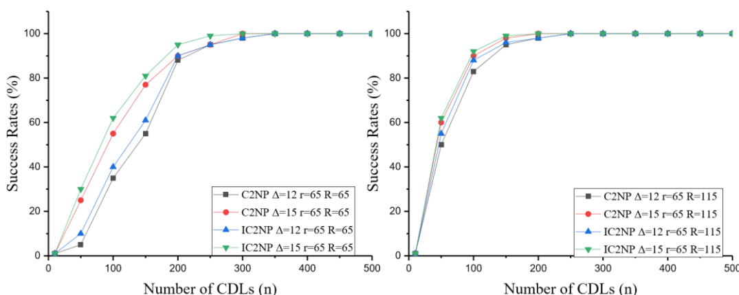
Figure 7. The success rate of C2NP and IC2NP (a) homogeneous scenarios
