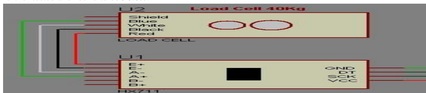
Figure 7. Load cell to HX711
