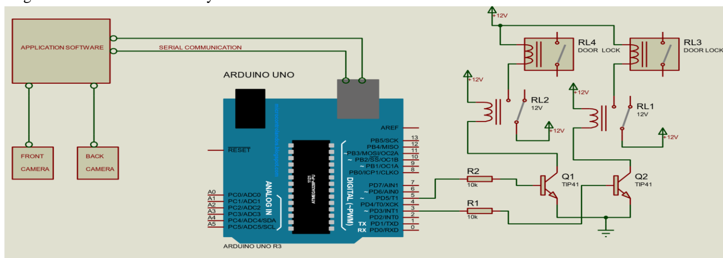
Figure 4. Access control circuit diagram
