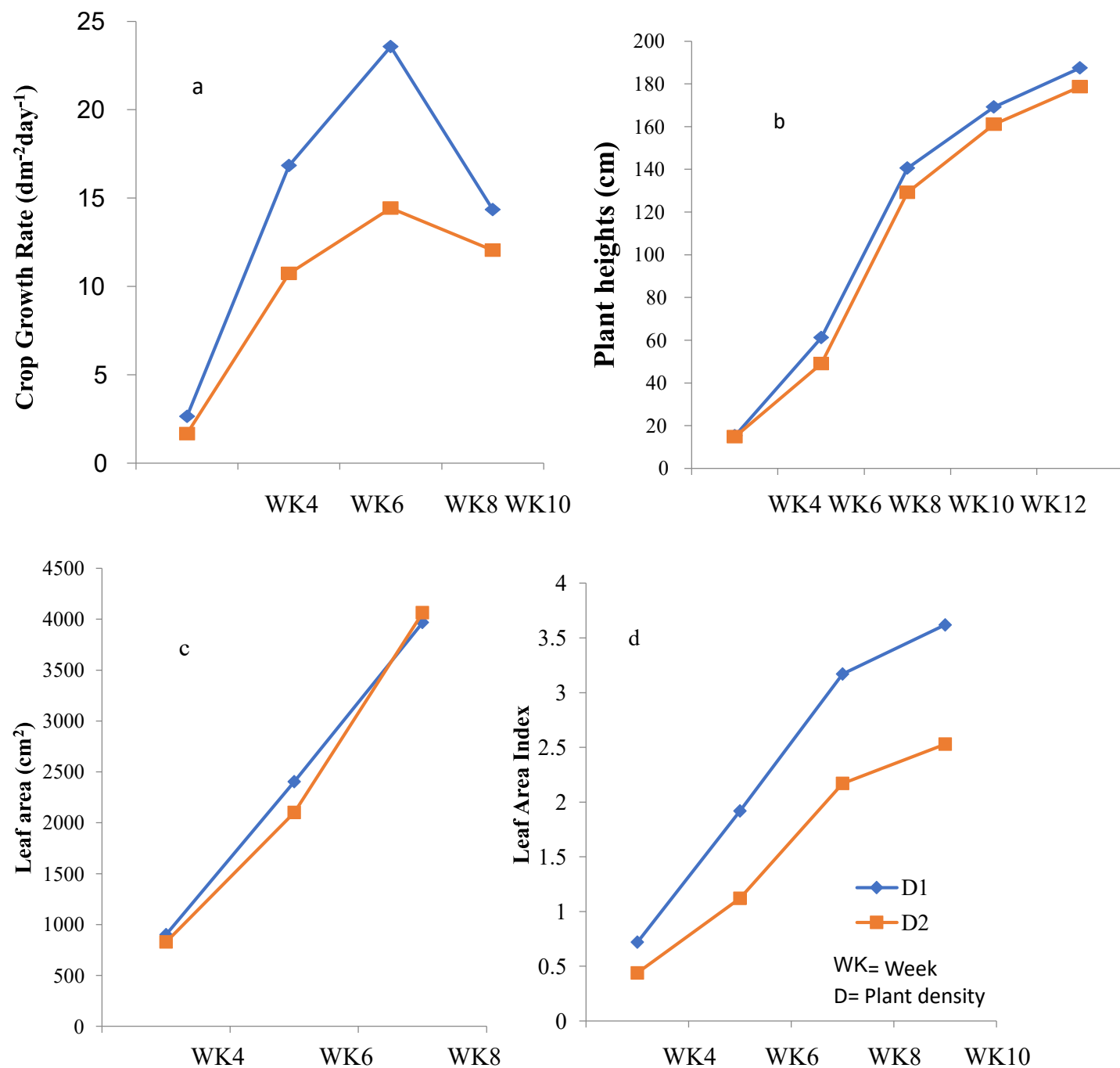
Figure 2: Effects of Plant density (D1=80,000; D2=53,333 plants per hectare) on weekly performances of plant heights, crop growth, leaf area and leaf area indices of four maize varieties grown in Ibadan
