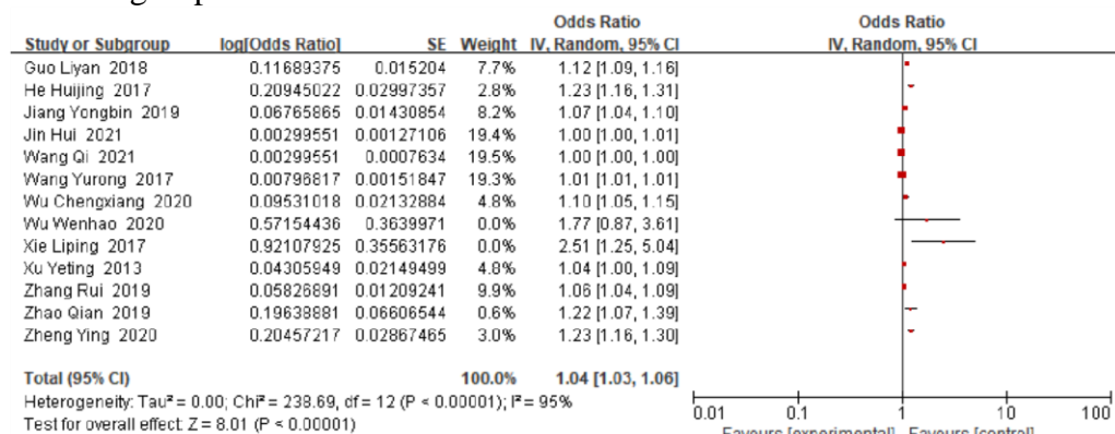
Figure 8: Forest map of diabetes course analysis
