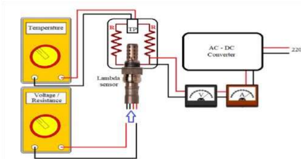
Figure 1 Figure used oxygen sensor
