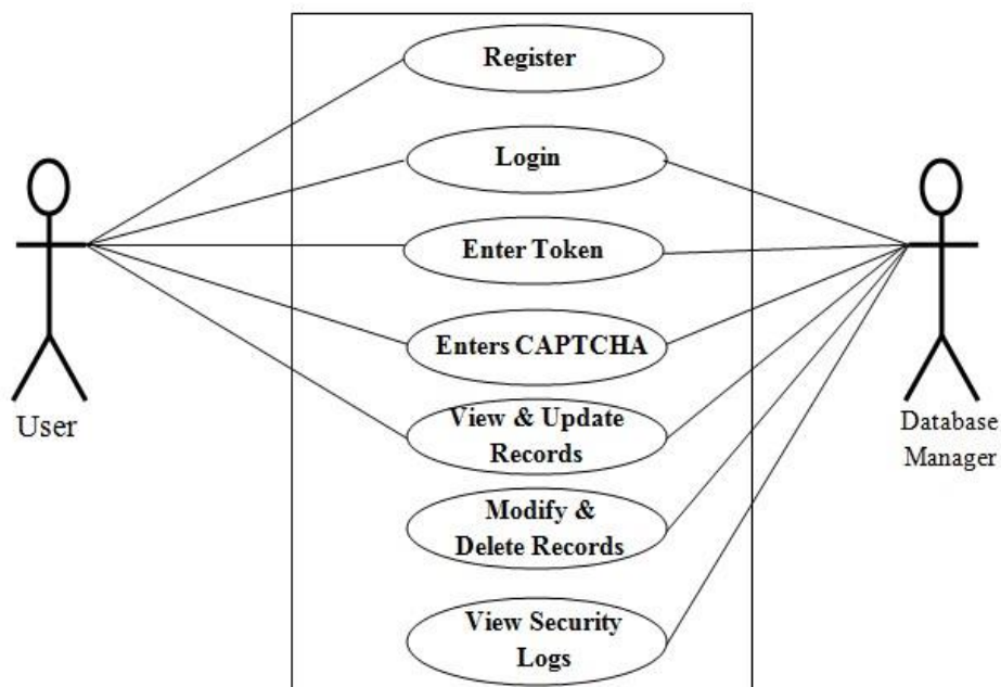
Figure 4.1: Use- case diagram of the proposed system
