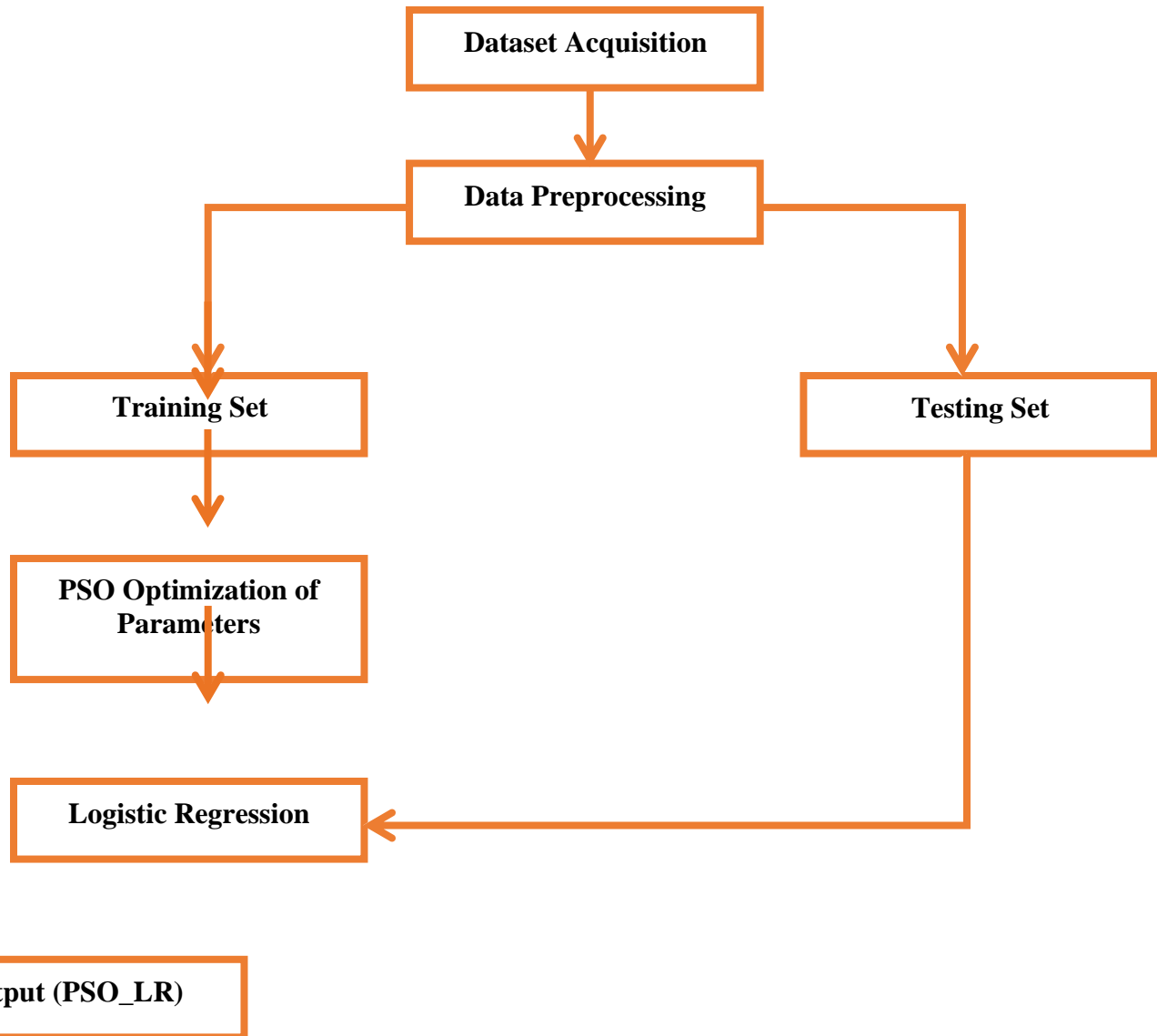
Fig 3.5: PSO-LR Flowchart
