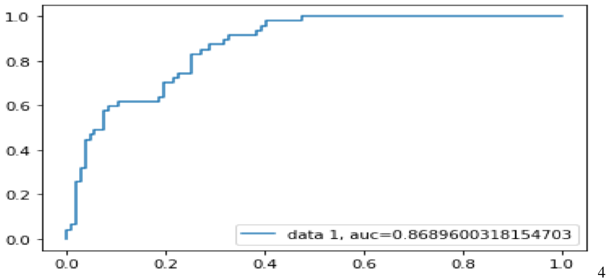
Fig.4.5: ROC Curve of Ordinary Logistic Regression
