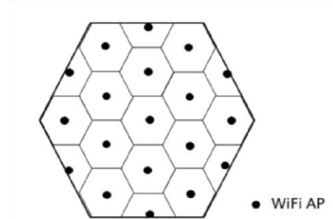
Fig. 1. An overlay network with K WiFi APs deployment covering a regular hexagonal LTE-A cell.
