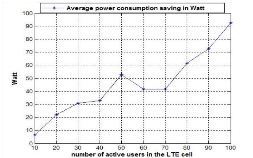
Fig. 6. Average Power Consumption saving in Watt.
