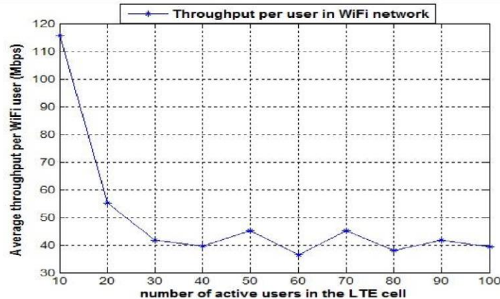
Fig. 4. Average per user WiFi throughput (Mbps)
