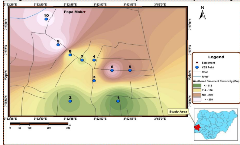
Figure 5: Isoresistivity map of weathered basement layer
