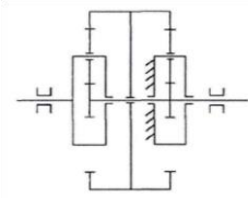
Figure 1: Planet carrier input + sun gear output
