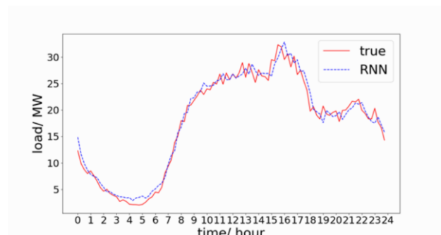
Figure 8: RNN prediction results
