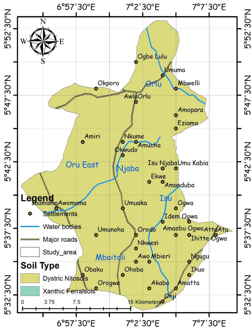
Figure 4: Spatial Distribution of Soil Types in the Study Area
