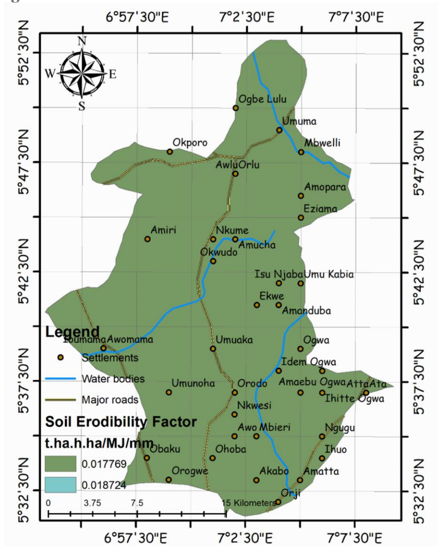
Figure 5: Spatial Distribution and Erodibility of Soil Types in the Study Area
