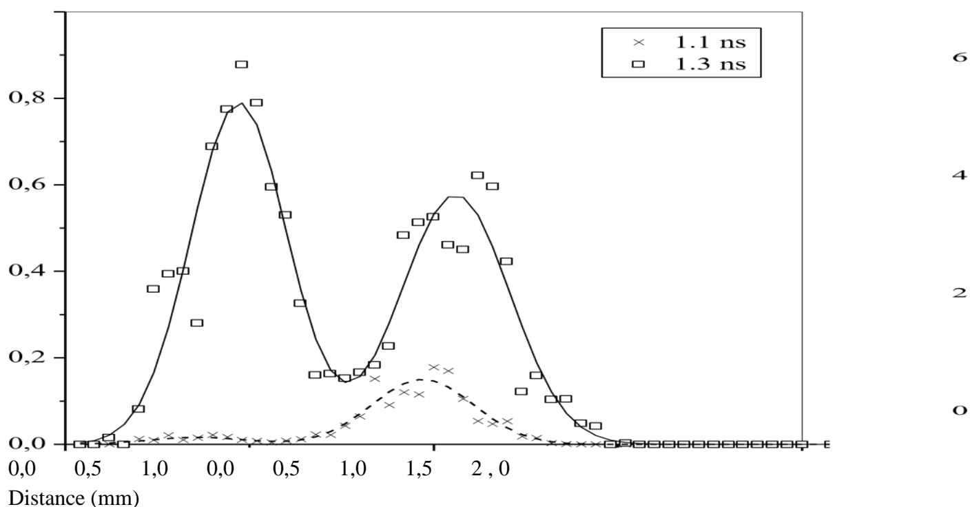
Fig. 17. Electron avalanches.Distance (mm)
