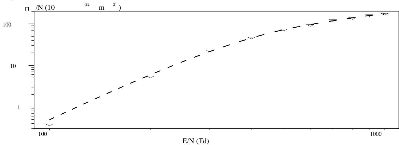
Fig. 8 Reduced ionization coefficient
