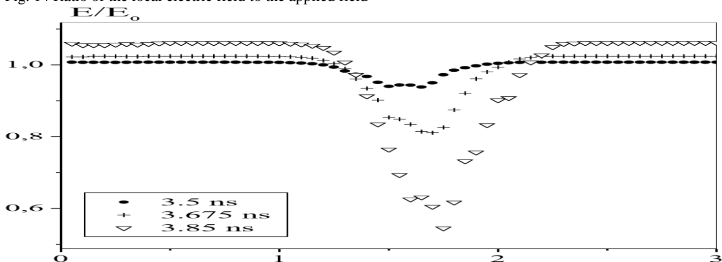
Fig. 14 Ratio of the local electric field to the applied field
