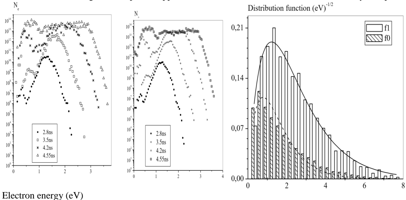
Fig. 9 Electron energy distribution at E/N=800 Td, f0: isotropic part, f1: with anisotropic parts.
