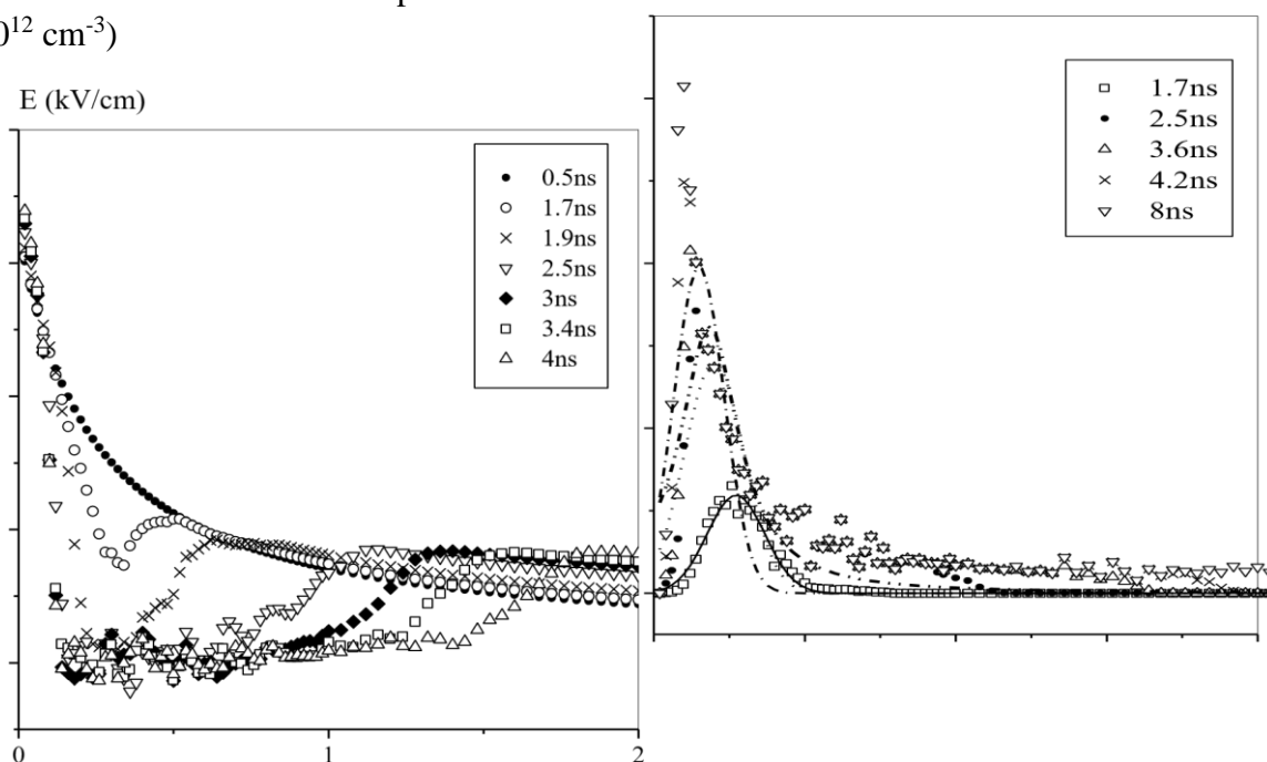
Fig. 17. Electron avalanches.Distance (mm)
