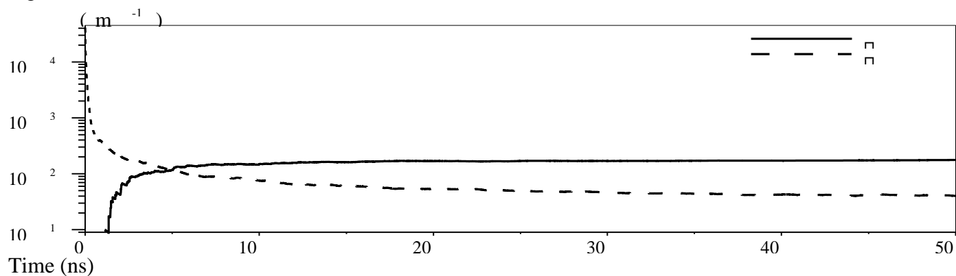
Fig. 3. Ionization ( \square ) and attachment ( \square ) coefficients for 500 Td
