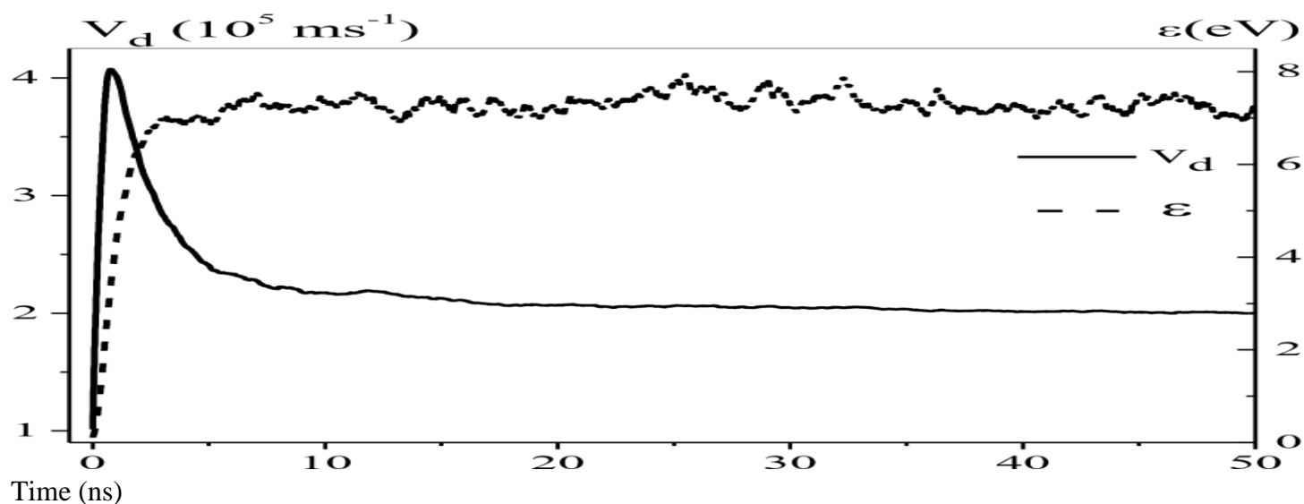
Fig. 1. Electron Drift velocity (W) and electron main energy ( \square ) for 300 Td
