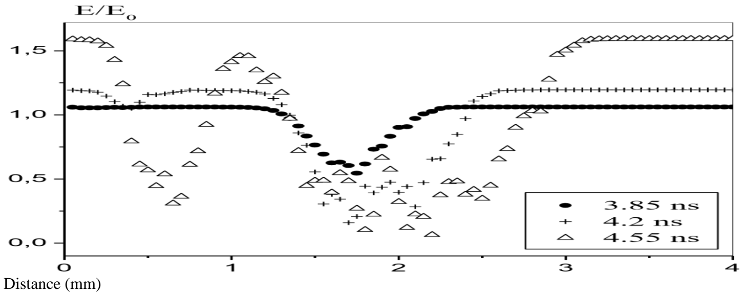
Fig. 16 Ratio of the local electric field to the applied field
