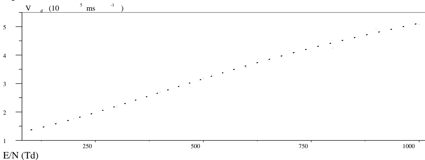
Fig. 5. Electron drift velocity
