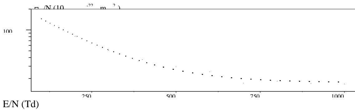
Fig. 7 Reduced attachment coefficient
