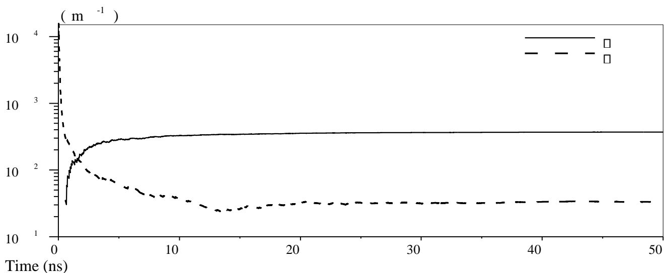
Fig. 4. Ionization ( \square ) and attachment ( \square ) coefficients for 700 Td
