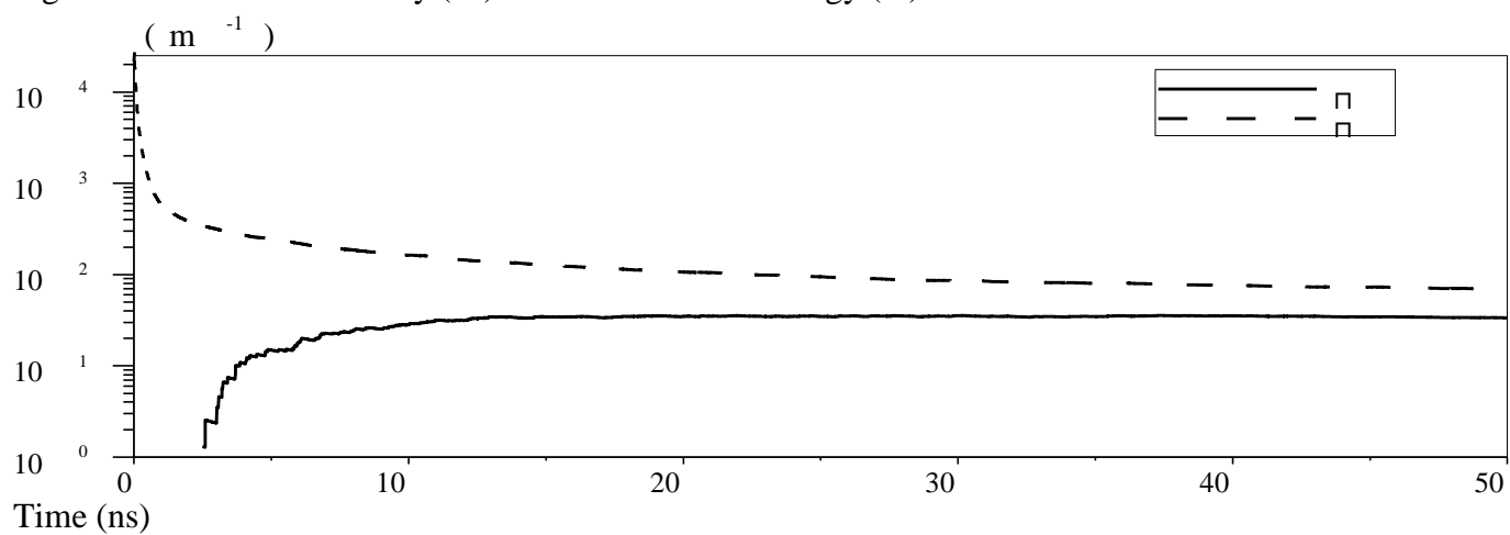
Fig. 2. Ionization ( \square ) and attachment ( \square ) coefficients for 300 Td
