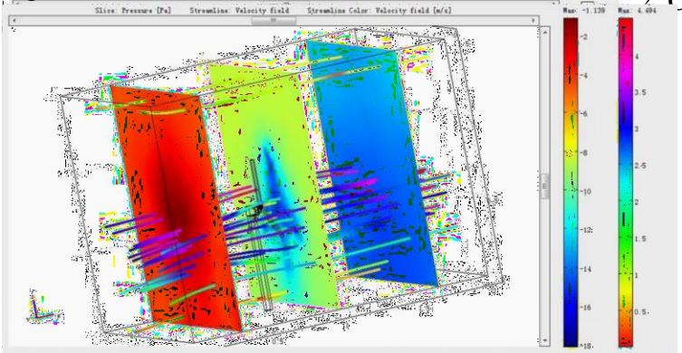
Figure 16 Pressure and streamline in 5 m/s maximum inlet speed in Case 2 Case 3 and Case 4
