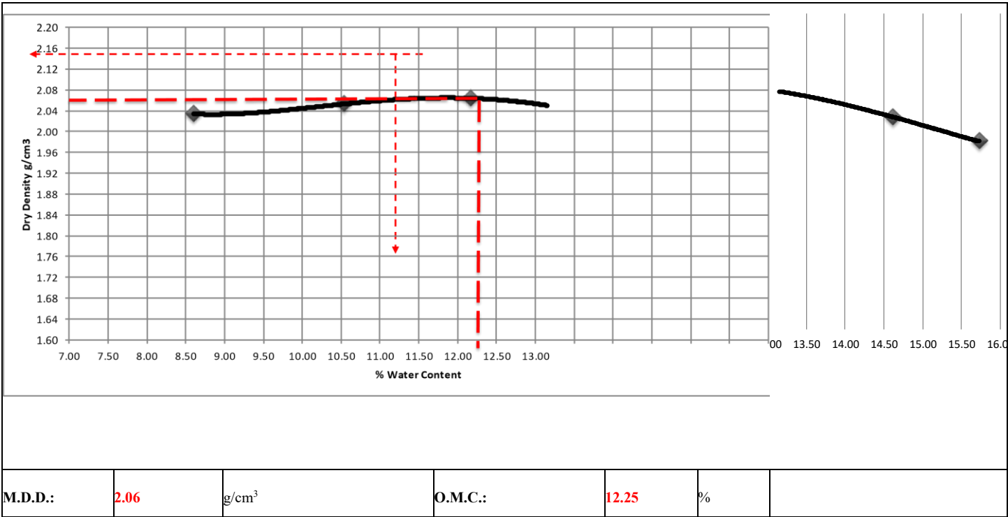
Fig. 14. A plot of dry density (mg/m^3) against water content (%) on compaction test (Point 5)
