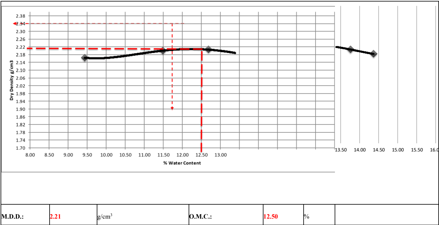
Fig. 8. A plot of dry density (mg/m^3) against water content (%) on compaction test (Point 3)
