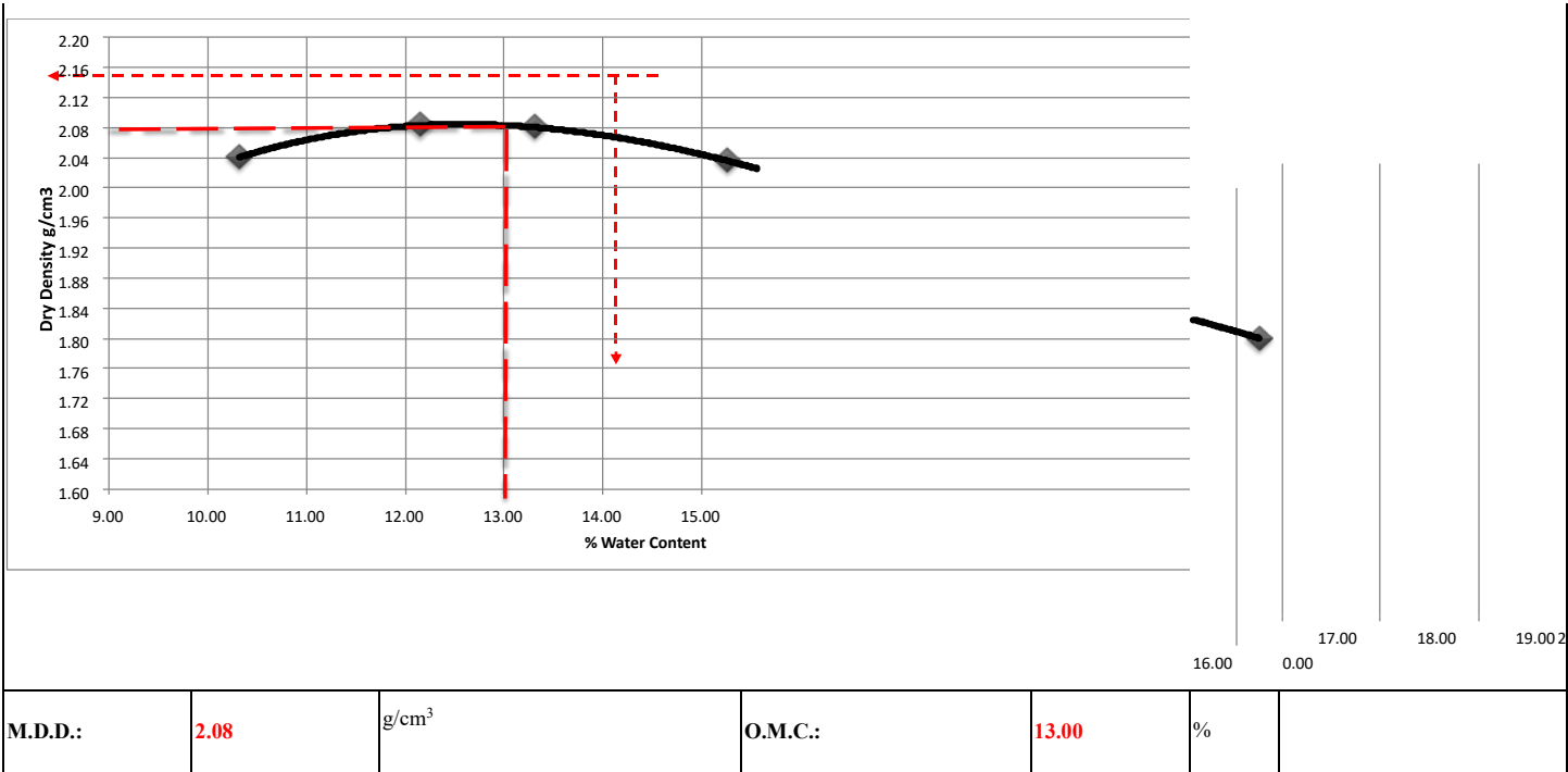
Fig. 11. A plot of dry density (mg/m^3) against water content (%) on compaction test (Point 4)
