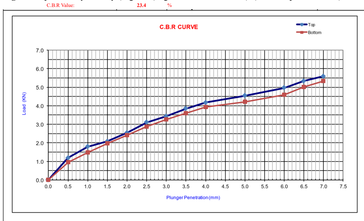
Fig. 18. A plot of load (KN) against plunger penetration (mm) on CBR test (SOAKED-24 HRS Point 6)
