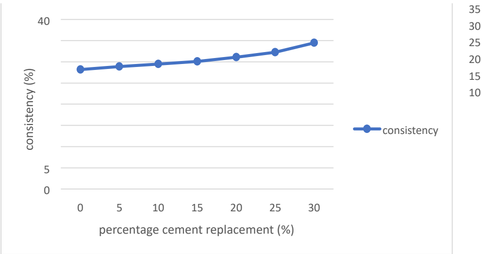
Figure 1. variation of consistency with percentage cement replacement
