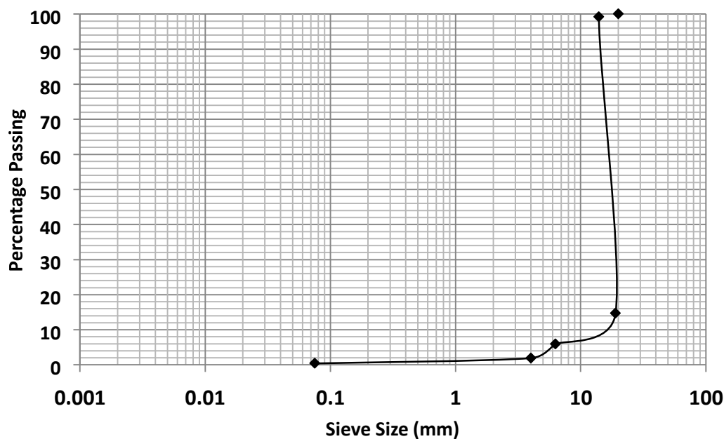
Figure 4. Particle size distribution of gravel
